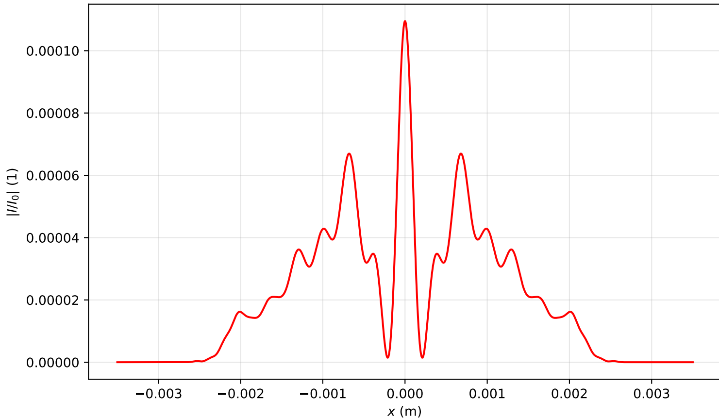
Intensity profile I(x, y = 0, z = 1.513)/I_0 , P_{in}=7.0P_{cr} , artificial time
